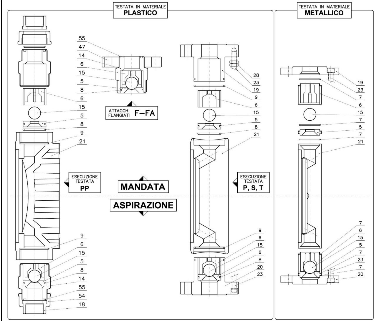
Figure 16 MAXIMUM PUMP FLOW RATE 600-1500 I/h: PUMP HEAD COMPONENTS
