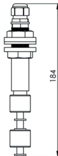
Fig. 7: Product tank dual level switch assembly
