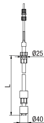
Fig. 7: Type SG-2 PVDF
