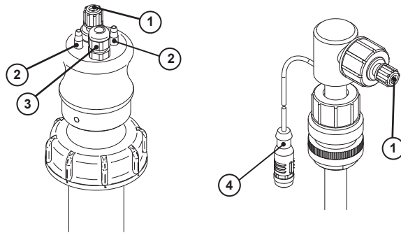
Fig. 14: Connection positions hydraulic installation
