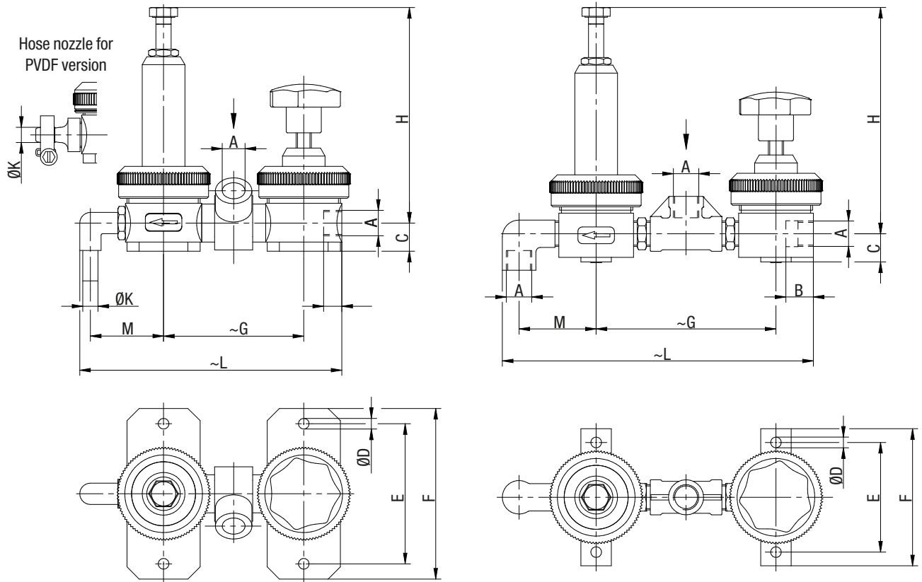
Fig. 7: Dimensioned drawing mounting block DN6
