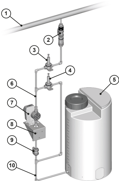
Fig. 9: Installation with a back-pressure valve and pressure-relief valve
