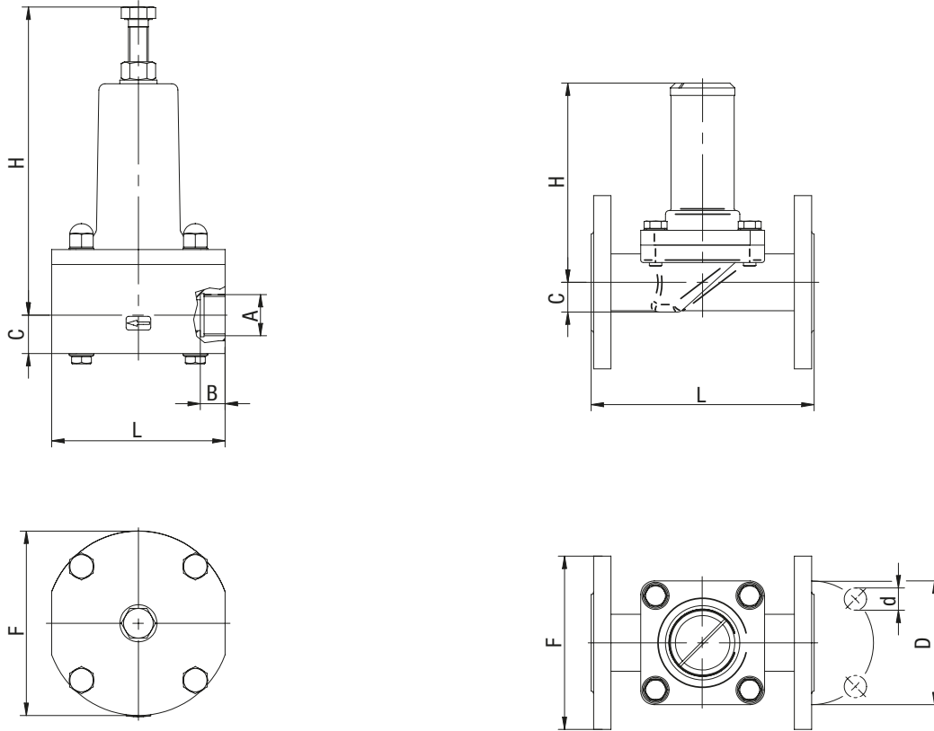
Fig. 3: Dimensioned drawing Back-pressure and pressure relief valves DN25 - DN65 (spring-loaded diaphragm valve)
