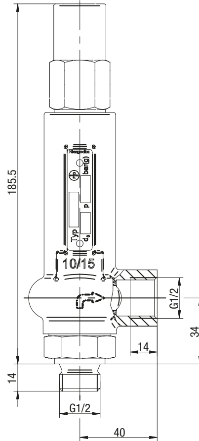
Fig. 5: Dimensioned drawing pressure-relief valve DN10 (spring-loaded seat valve)
