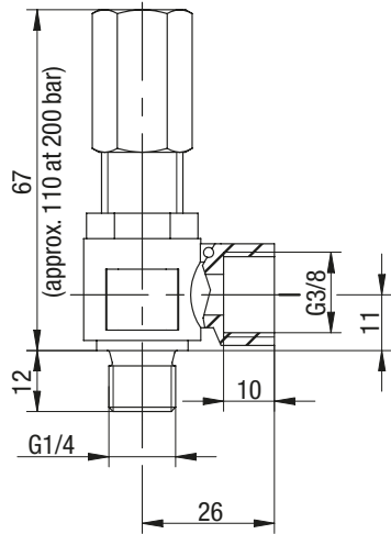
Fig. 4: Dimensioned drawing pressure-relief valve DN6 (spring-loaded seat valve)
