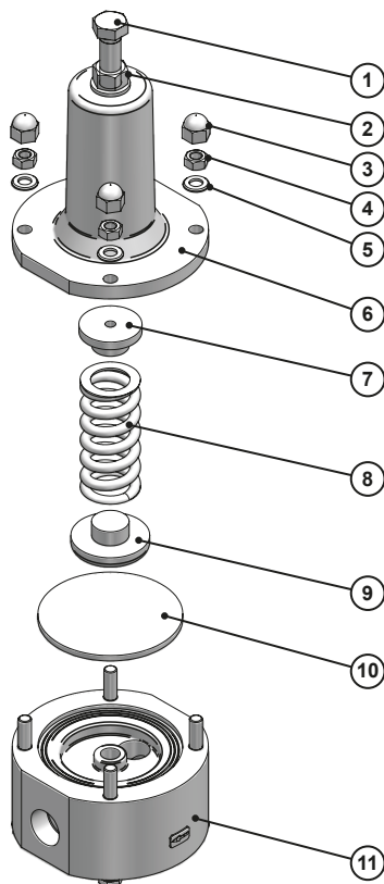
Fig. 13: Exploded diagram of the back-pressure and pressure-relief valves DN25 - DN65
