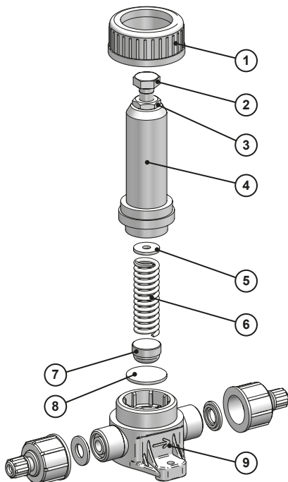
Fig. 11: Exploded diagram of the back-pressure and pressure-relief valves DN6 - DN15
