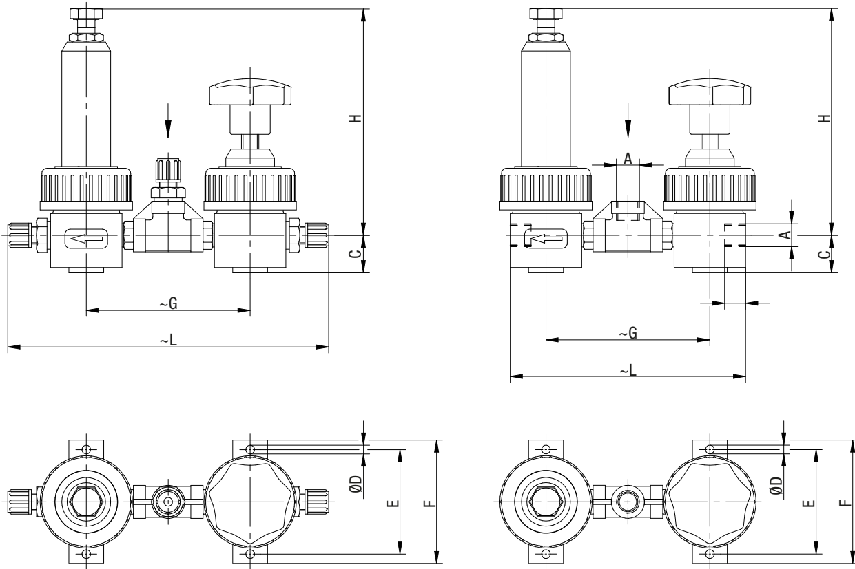
Fig. 6: Dimensioned drawing mounting block DN6
