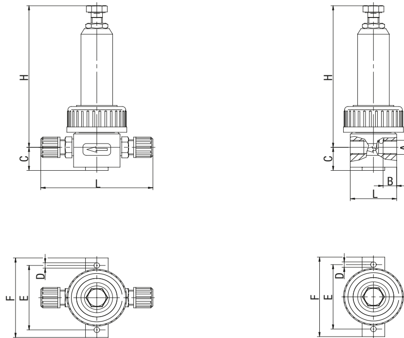
Fig. 2: Dimensioned drawing Back-pressure and pressure relief valves DN6 - DN15 (spring-loaded diaphragm valve)
